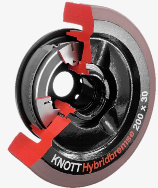
Hybrid Brake
